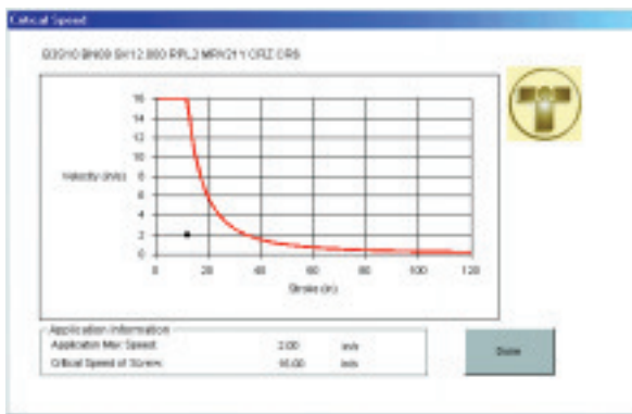
THE CRITICAL SPEED WINDOW SHOWS THE APPLICATION'S MAXIMUM SPEED, RELATIVE TO CRITICAL SPEED OF THE SCREW.
